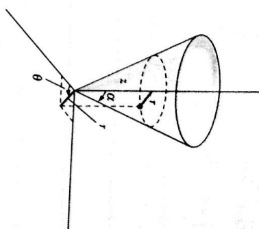
FIGURE 7.2 Example 7.4. A smooth cone of half-angle \alpha . We choose r , \theta , and z as the generalized coordinates.
