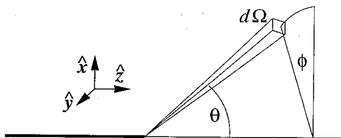
Figure 2.1: Geometry of a scattering process.
