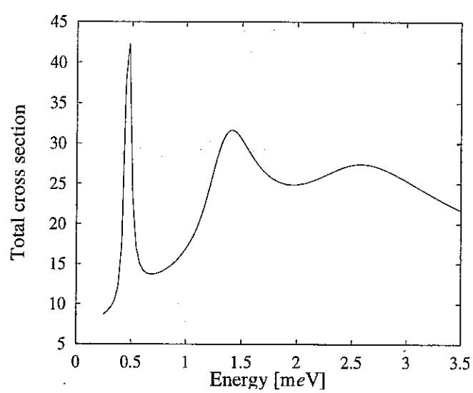
Figure 2.4: The total cross section shown as function of the energy for a Lennard-Jones potential modeling the H-Kr system. Peaks correspond to the resonant scattering states.
