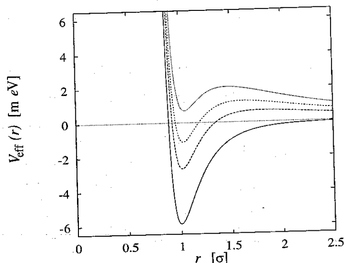
Figure 2.3: The effective potential for the Lennard-Jones interaction for various l -values.
