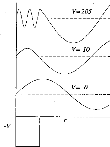
Figure 2.2: The radial wave functions for l=0 for various square well potential depths.
