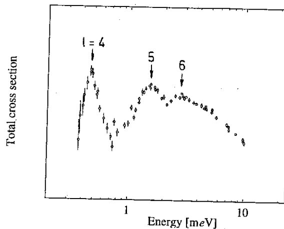
Figure 2.5: Experimental results as obtained by Toennies et al. 7 for the total cross section (arbitrary units) of the scattering of hydrogen atoms by krypton atoms as function of centre of mass energy.
